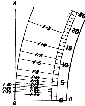
Fig. 72a.—Angles and degrees compared. It will be observed that an angle of 1 in 4 is practically 14°.
